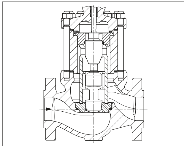
Fig. 4: Type 261GR Globe Valve with 4-stage CDST plug
