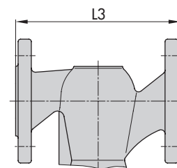
Flanged body (DN 32, 40, and 50)
