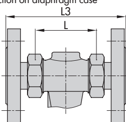
With flanges
